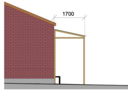
② New Shelter Section 1:25
